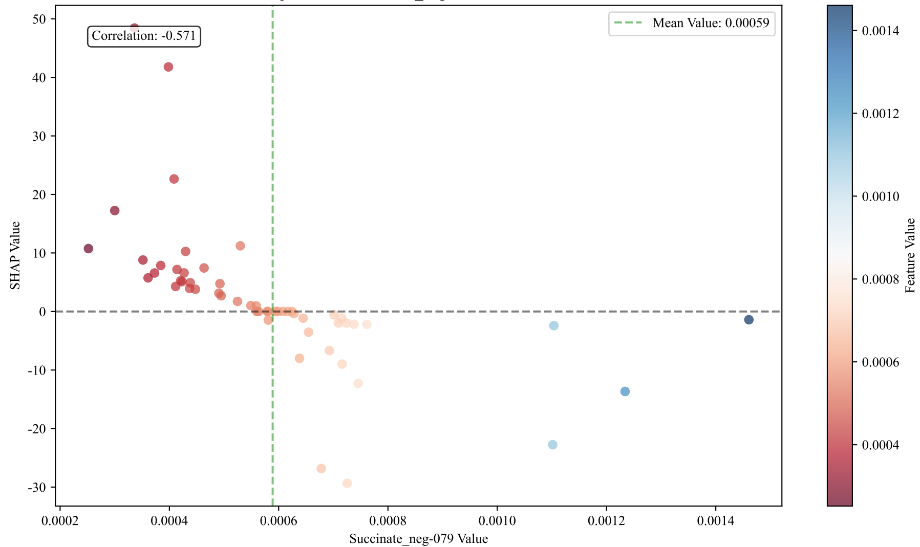
Relationship between Succinate_neg-079 Value and SHAP Value
